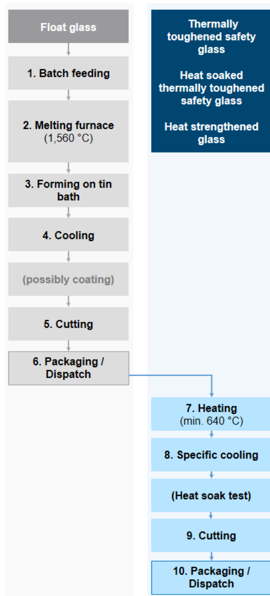
Illustration 1 Manufacturing process
