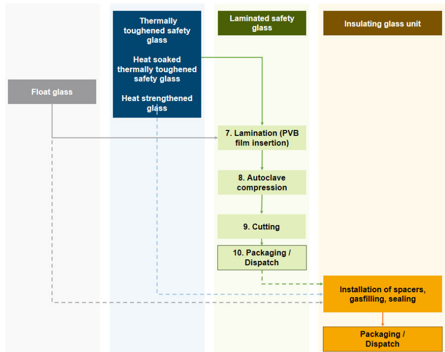
Illustration 1 Manufacturing process
